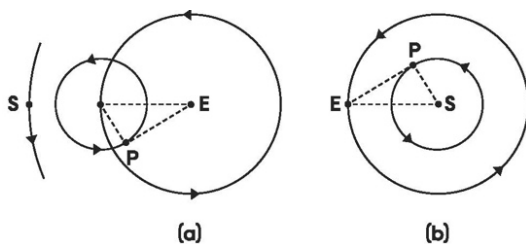
Figure 1: maximum elongation as accounted for in the Ptolemaic and the Copernican model (a and b, respectively). From Kuhn (1957).
